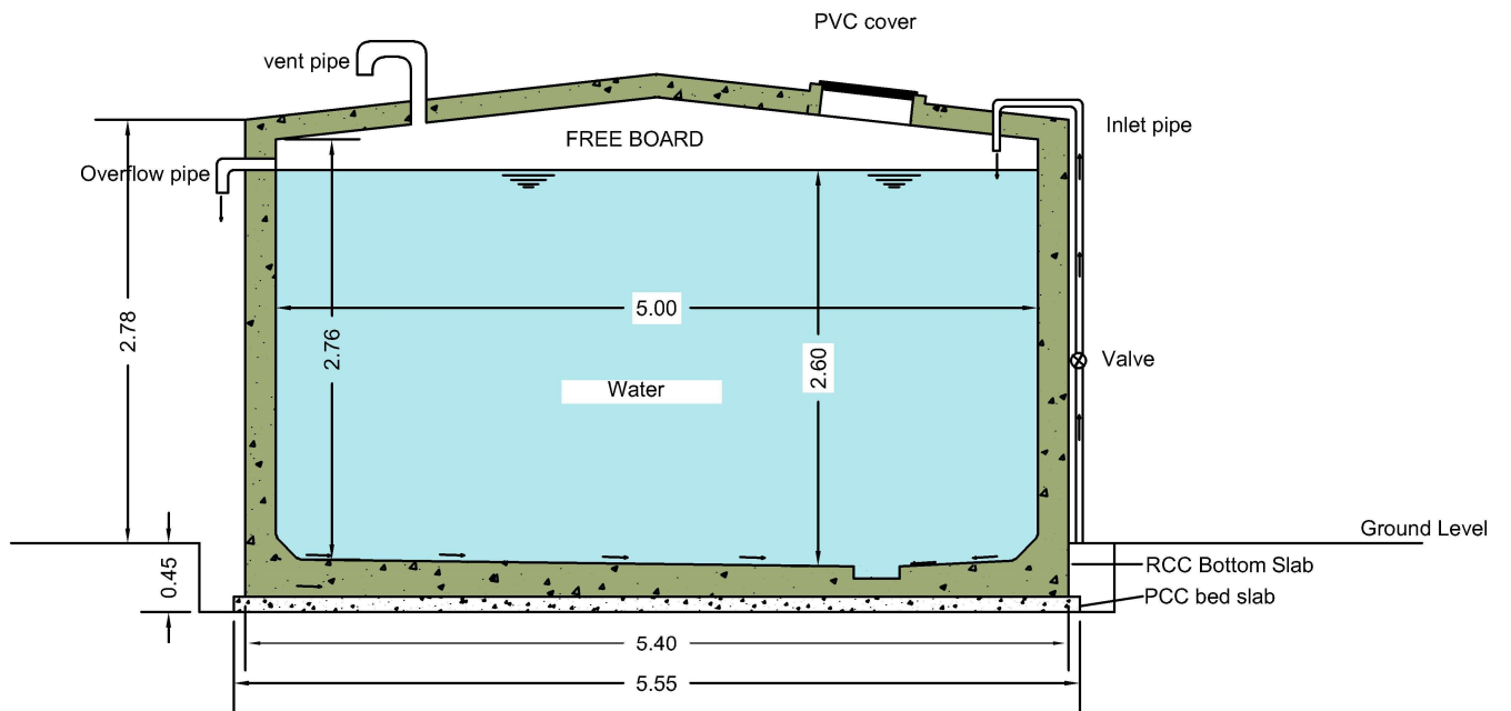
SECTION X-X
